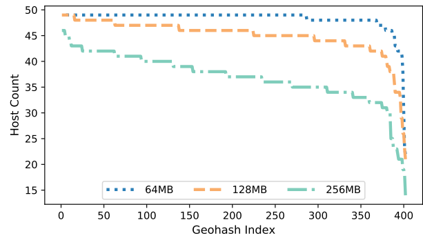
Figure 5: Depiction of the number of hosts that each unique geohash is present on after 1TB of data is inserted in a 50 node Atlas cluster. Highlights the effectiveness of Atlas’ data dispersion policies.
