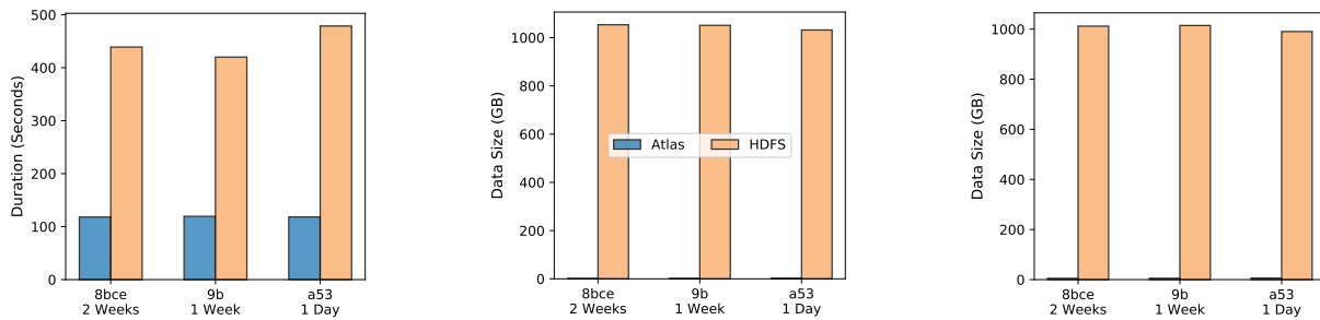
(a) Duration of spatiotemporal histogram analytics. Atlas reduces by up to 4x compared to canonical HDFS.
